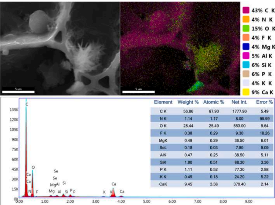
Fig. 17. EDX of washed unearthed biochar.
